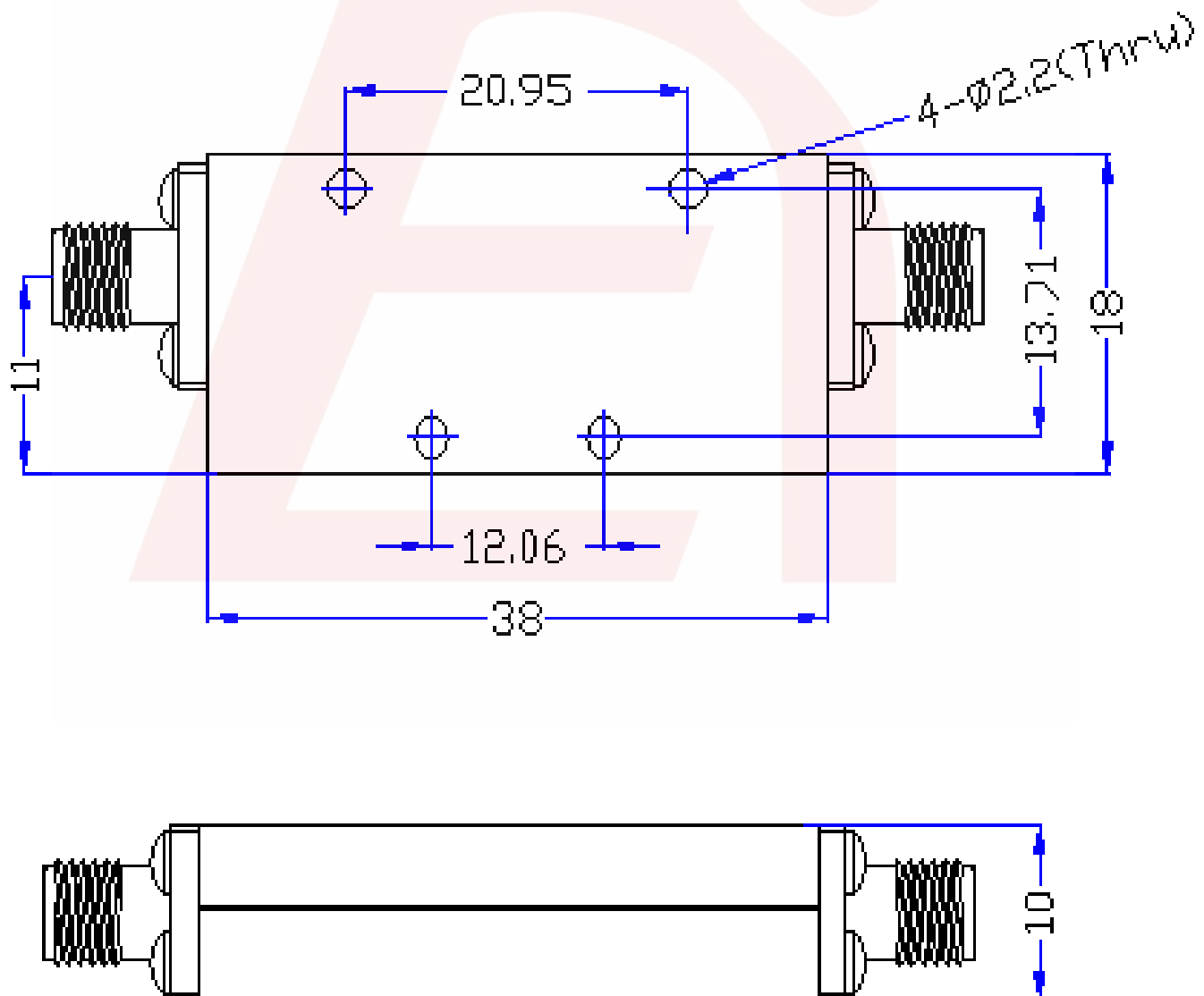
Outline Drawing:
