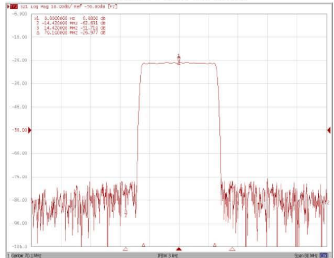
Attenuation Fo±14.42MHz
