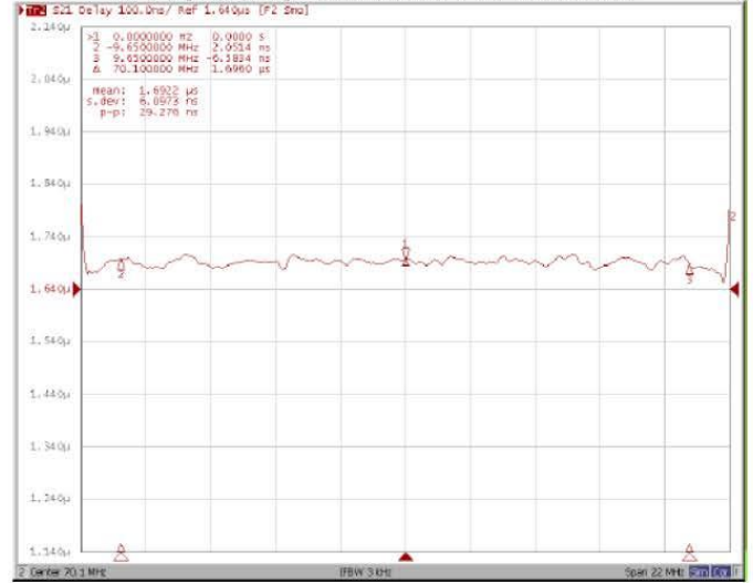
Group Delay Variation Fo±9.65MHz
