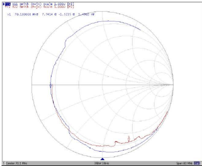
Smith Chart
