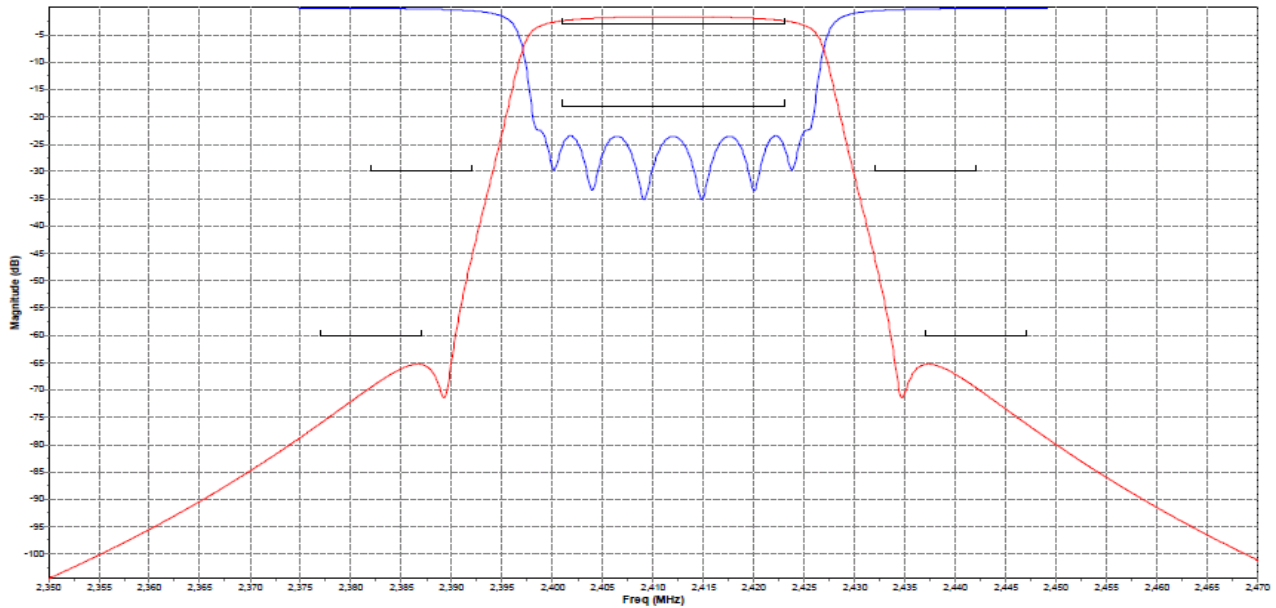
Fig.1 Return Loss and Rejection
